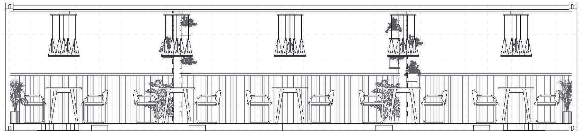
front elevation 40'
