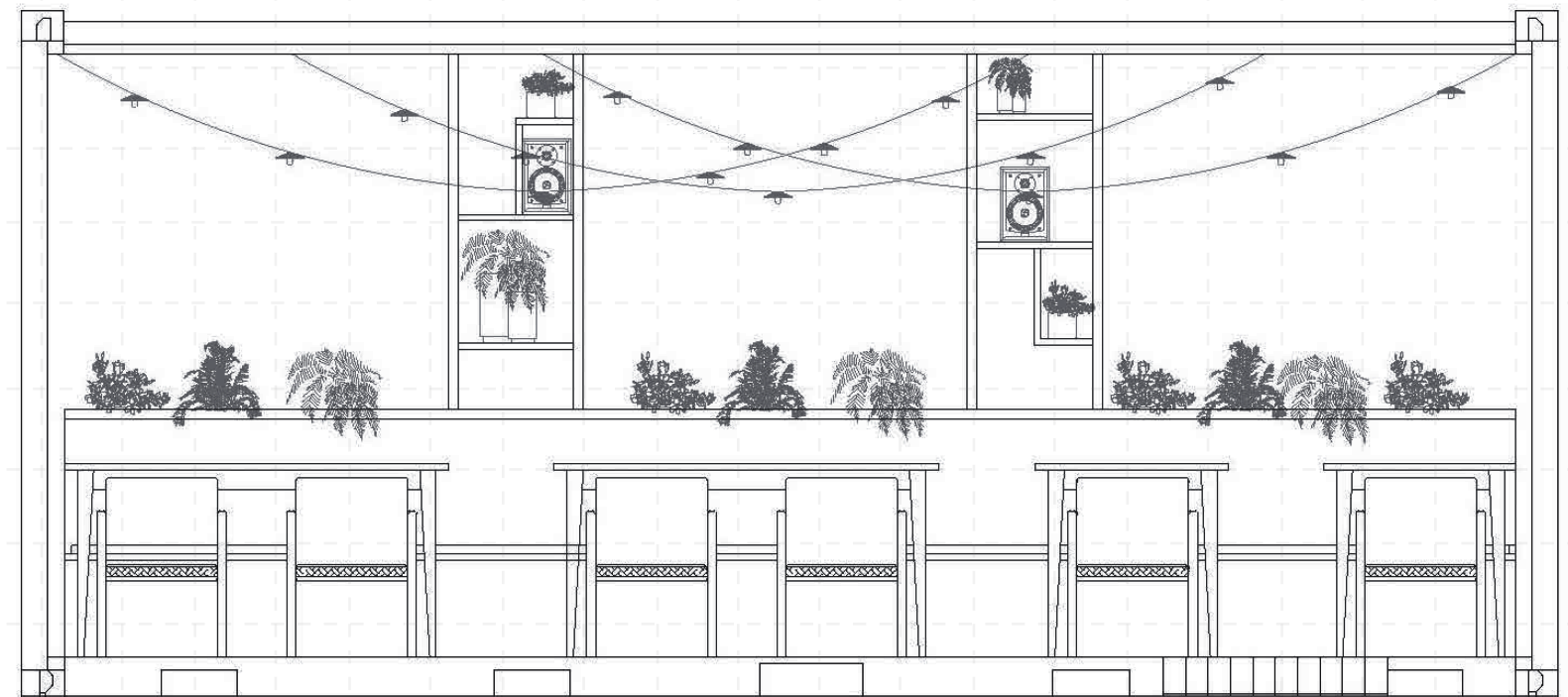
front elevation 20'
